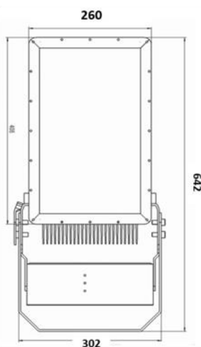
UN602-SL 100W/200W
