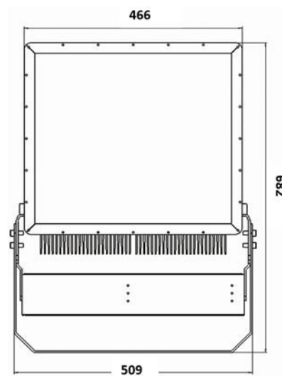
UN602-SL 300W/400W
